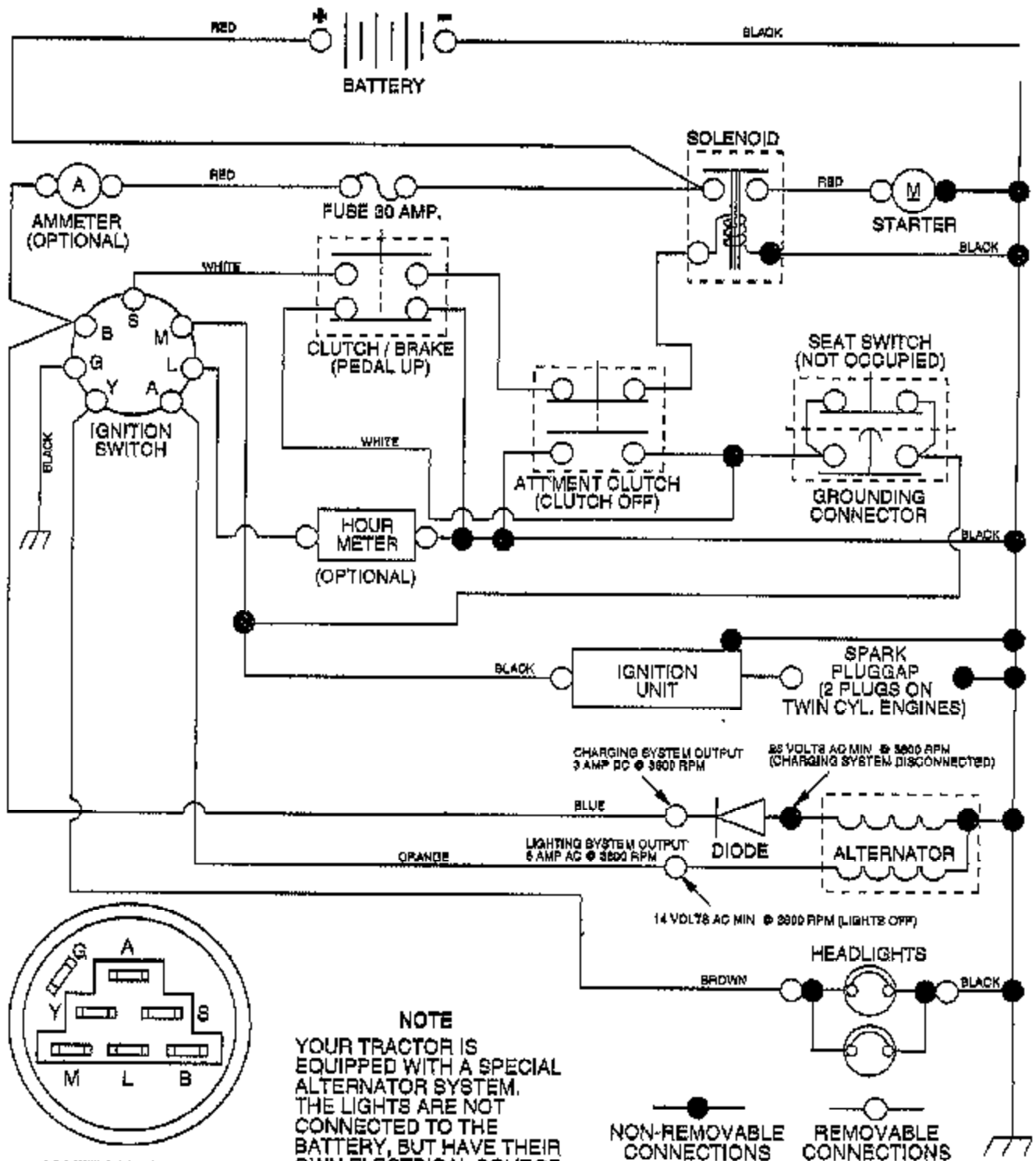
IGNITION SWITCH
