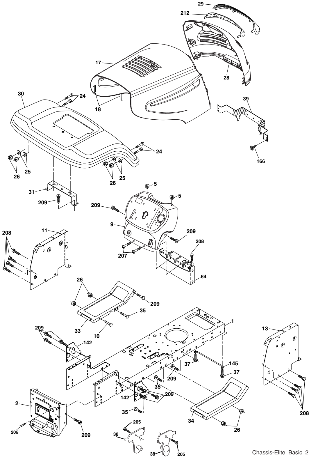
Chassis-Elite_Basic_2
