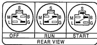
IGNITION SWITCH
